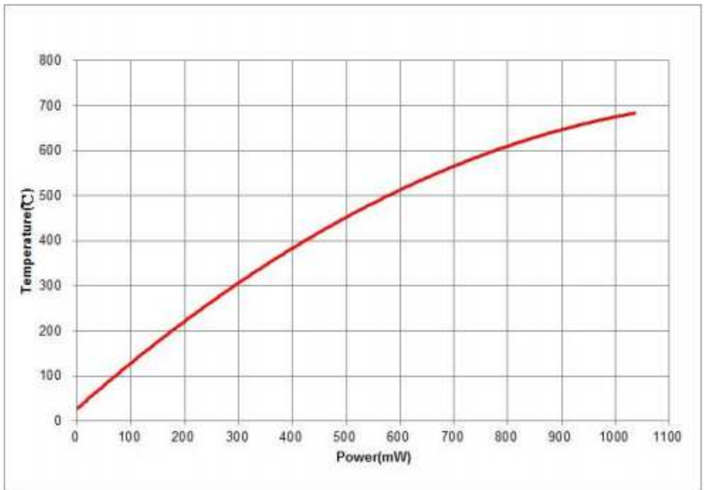
Typical Temp-Power Curve
