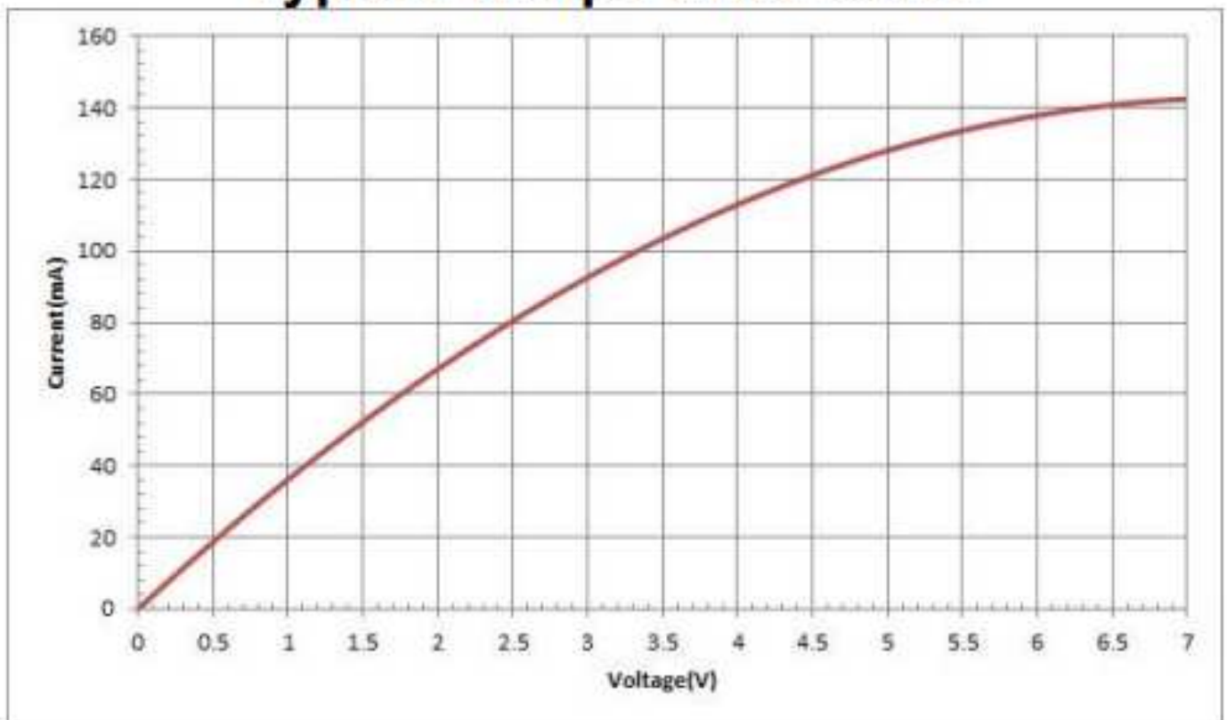
Typical I-V Curve
